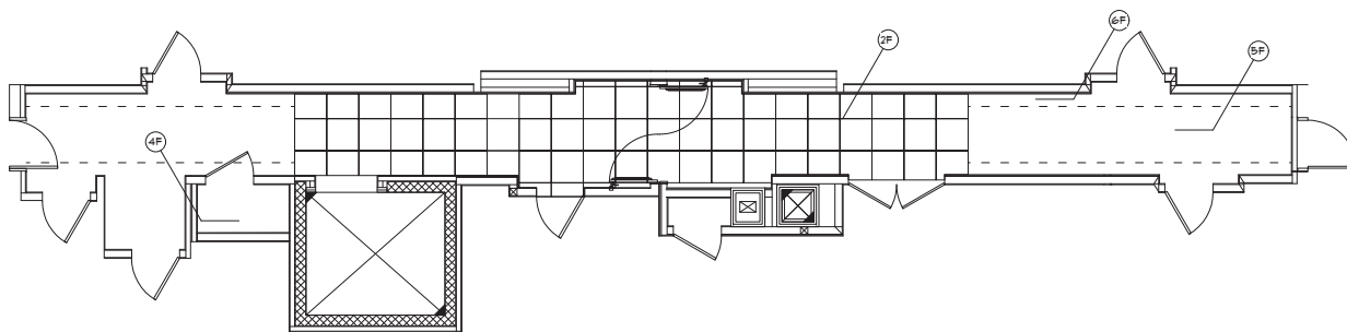
SECOND FLOOR CORRIDOR FINISH PLAN
