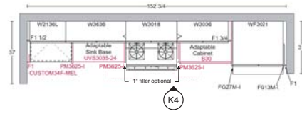
KITCHEN PLAN
