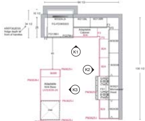
KITCHEN PLAN
