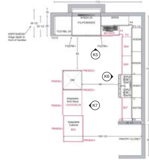
KITCHEN PLAN
