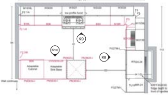
KITCHEN PLAN
